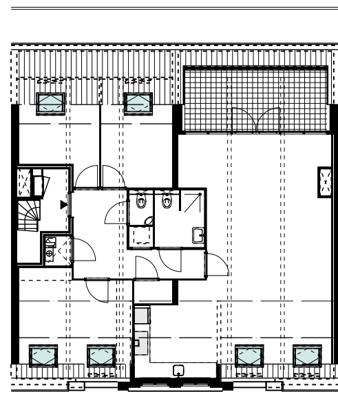
Zolder
