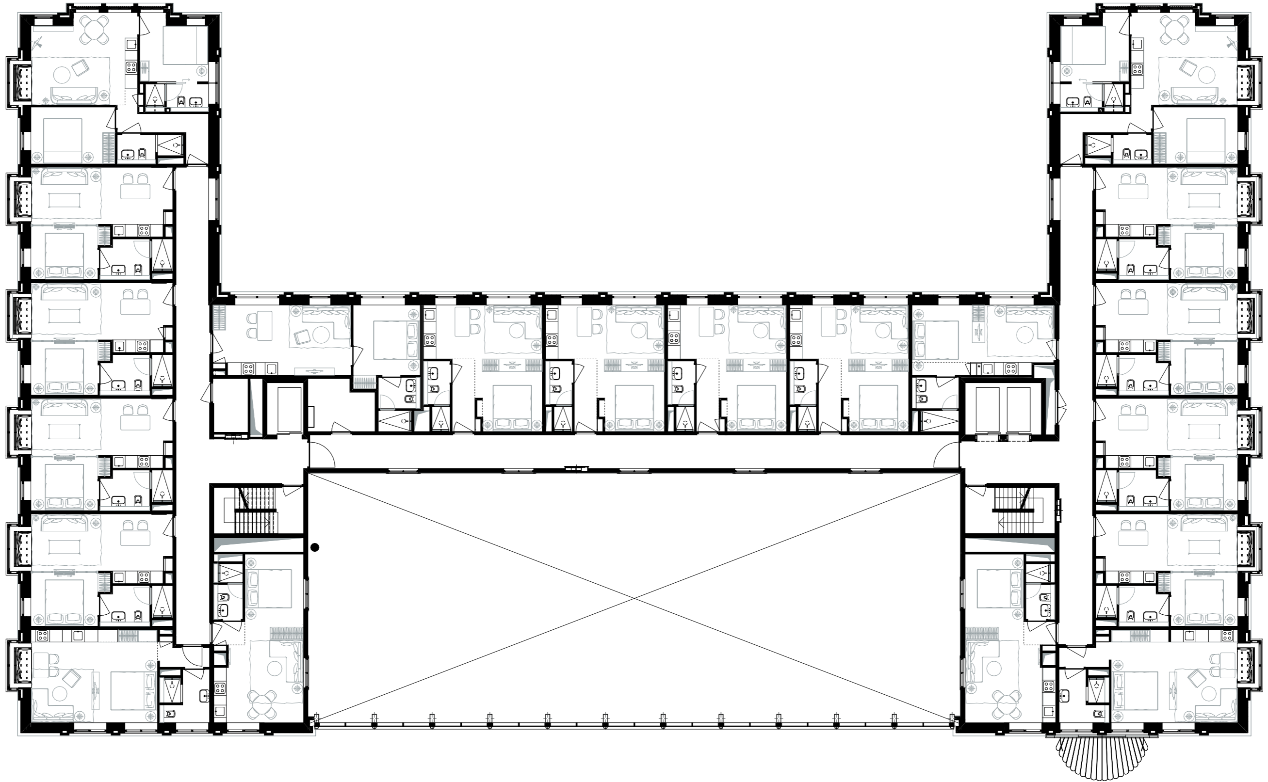
Boat & Co, Houthaven Amsterdam Floor levels 1 - 3
