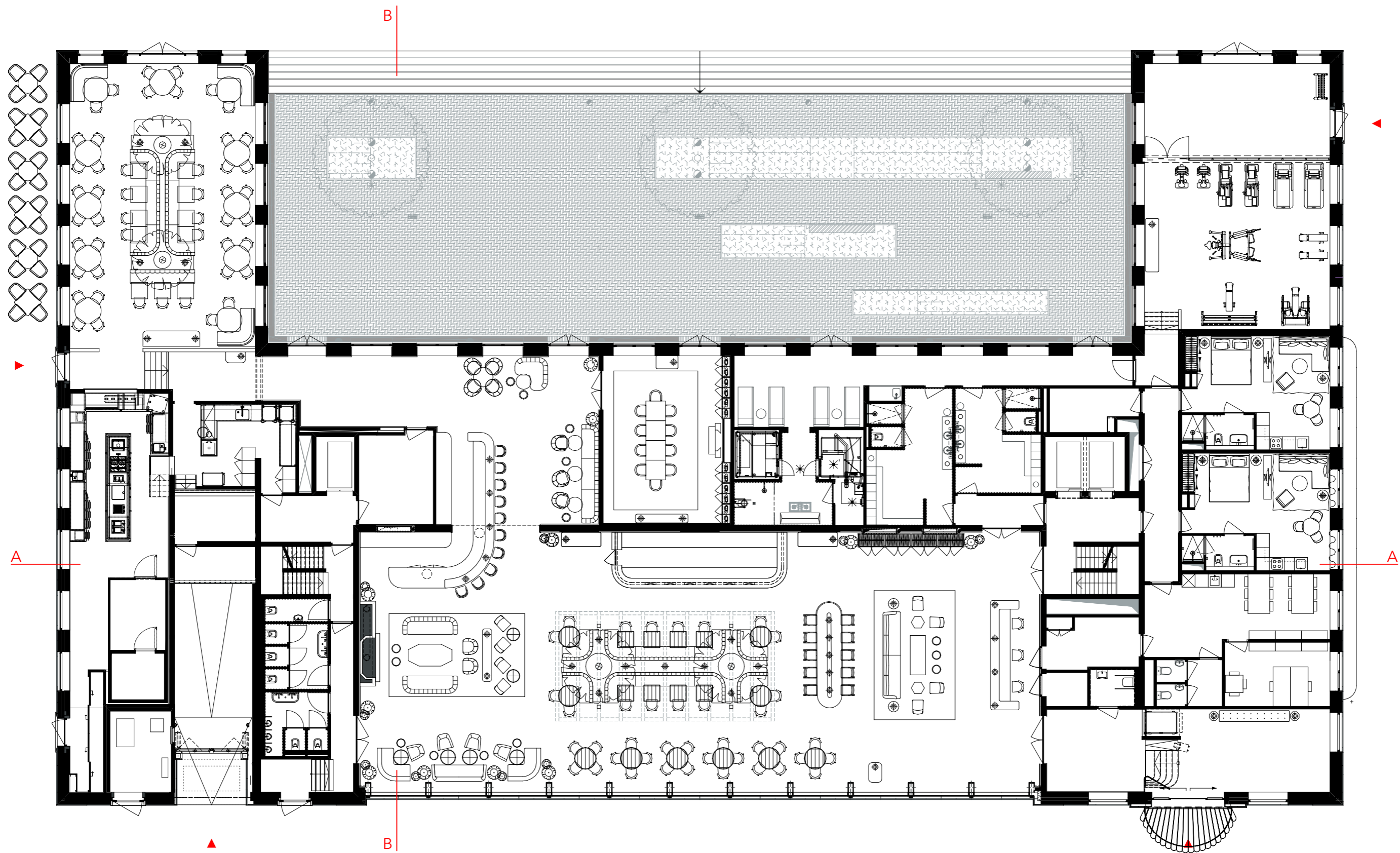
Boat & Co, Houthaven Amsterdam Ground floor
